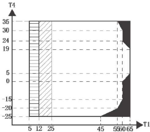
Figure 2-5.1: Heating operating limits 1
