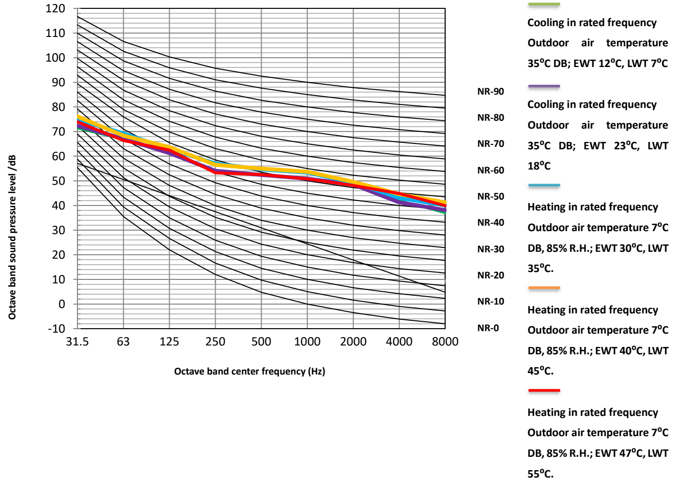
Figure 2-7.7: KHC-16RY3-B octave band levels
