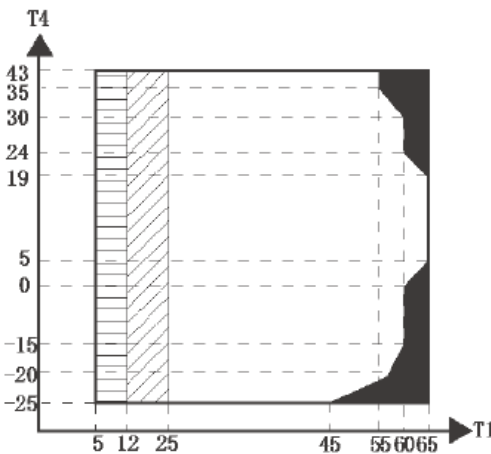
Figure 2-5.3: Domestic hot water operating limits 1
